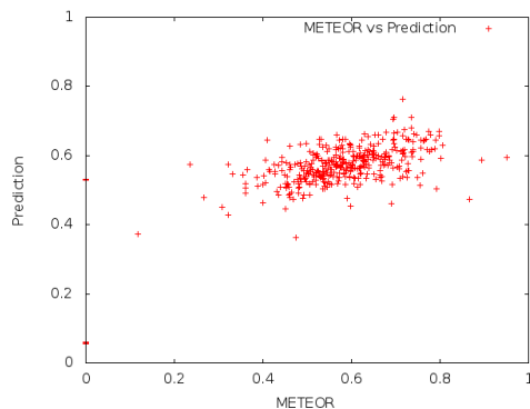
Figure 4: Expected versus predicted METEOR scores
